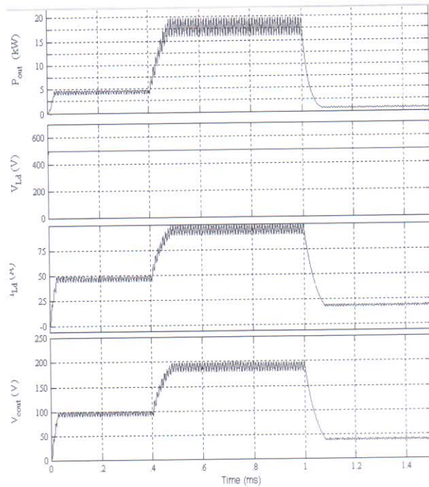
Fig. 6. Figure showing simulation results –(a) variation in output power obtained with time according to command signals (b) Voltage waveform across the resistive load (c) Variation in load current as per command (d) Variation in voltage across output capacitor.
