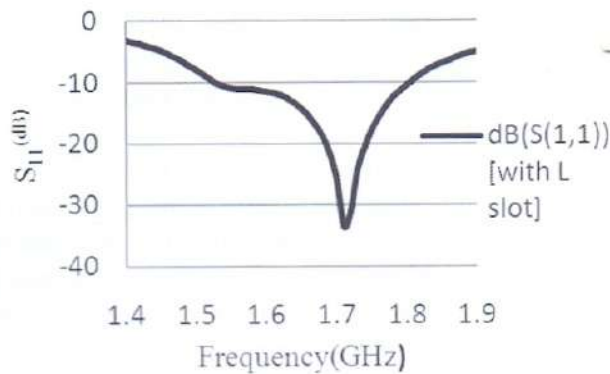
Fig. 2 Simulated return loss
