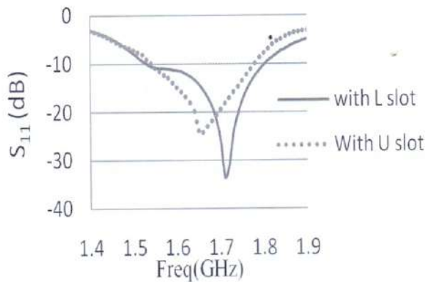
Fig.9 Comparison of return loss with different U/L slot
