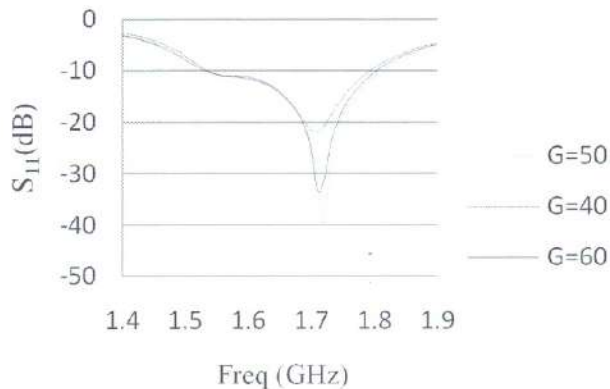
Fig. 5 Measured return loss with different size of ground plane with L slot
