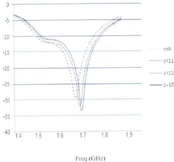
Fig.8 Simulated return loss with different size of ground plane
