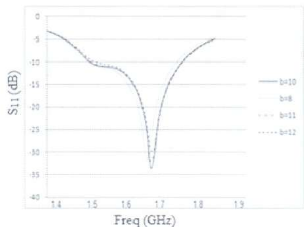
Fig. 7 Simulated Return loss with different size of b
