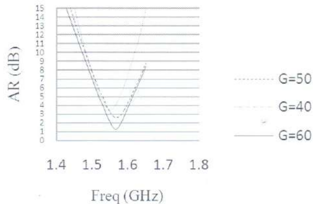
Fig.6 Axial ratio with different size of ground plane
