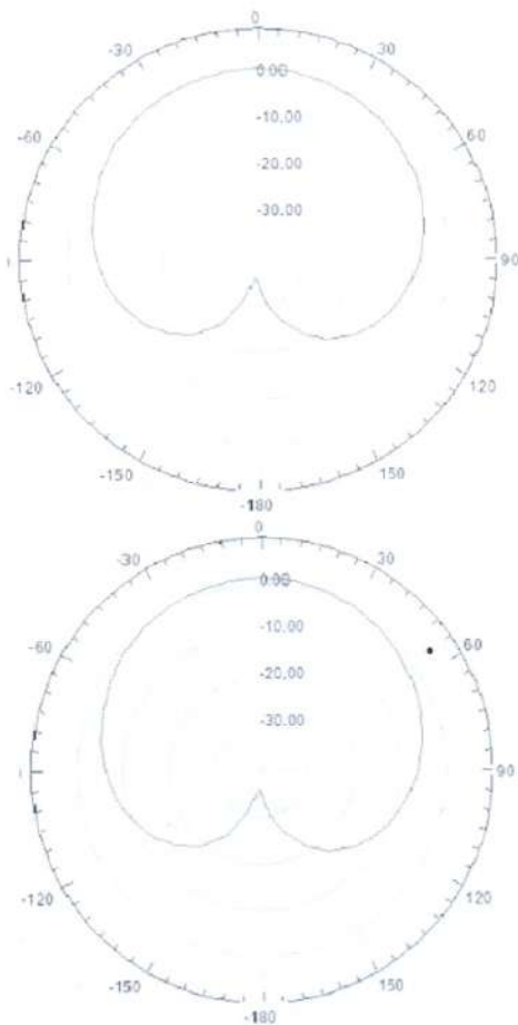
Fig.3 LHCP Radiation pattern at 1.575 GHz ( \Theta=90^\circ, 0^\circ )
