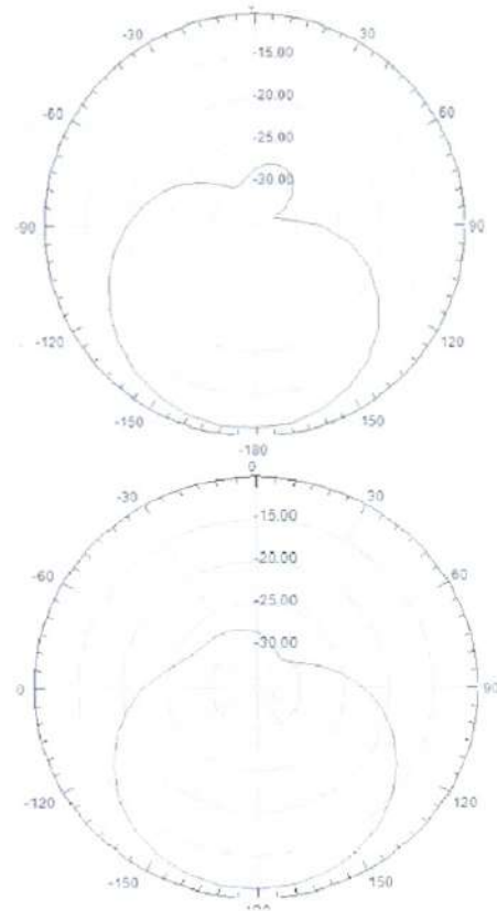
Fig. 4 RHCP Radiation pattern at 1.575 GHz ( \Theta=90^\circ, 0^\circ )
