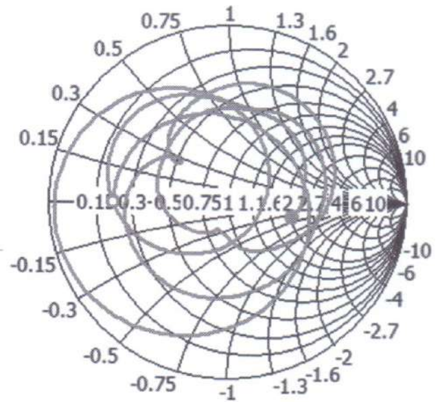
Figure 4 (l) Z Smith Chart
