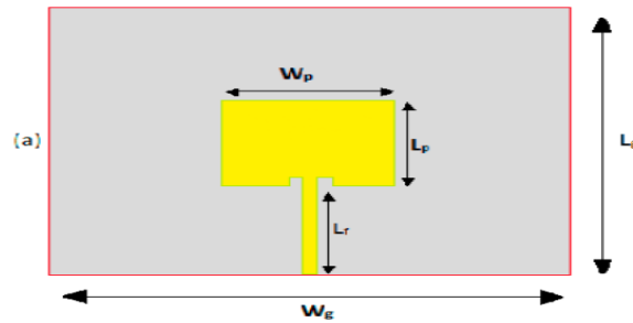
Fig. 1(a) The top view of designed antenna.
