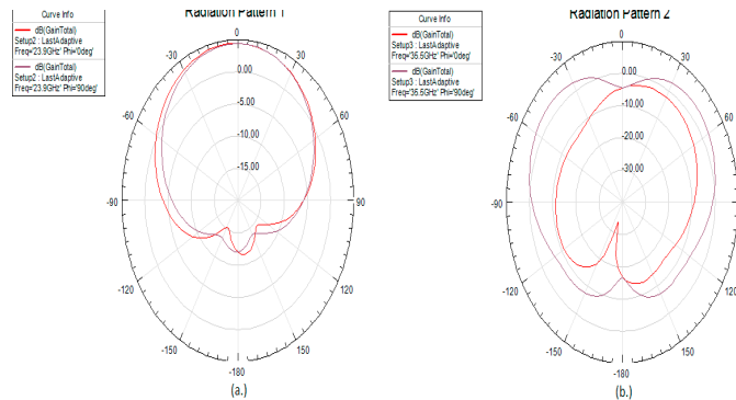
Fig.5 Radiation pattern sweep in 360°angle
