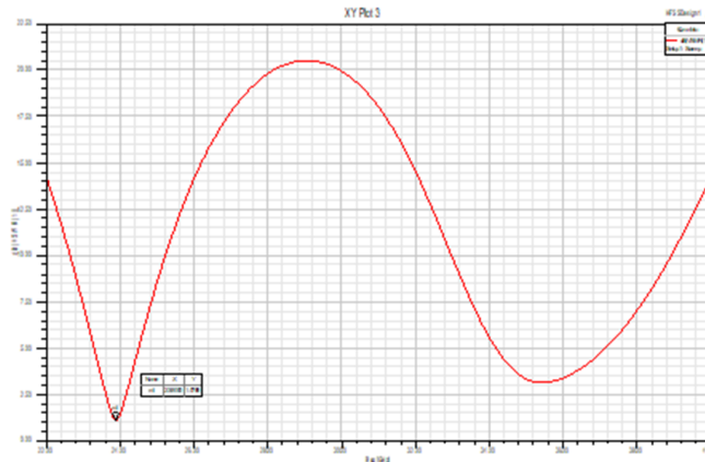
Fig. 4. VSWR of the antenna
