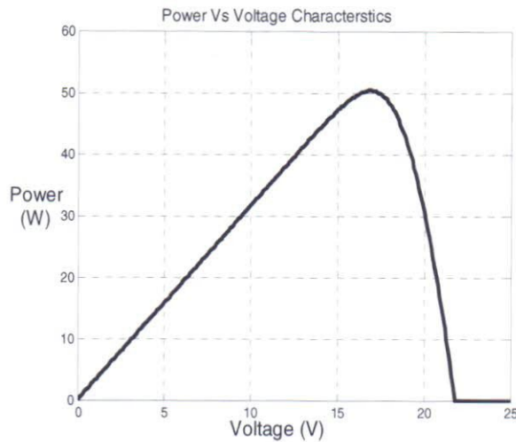
Fig.3 Characteristics of BP 350 solar module at insolation 1000\text{W/m}^2 at 25^\circ\text{C}
