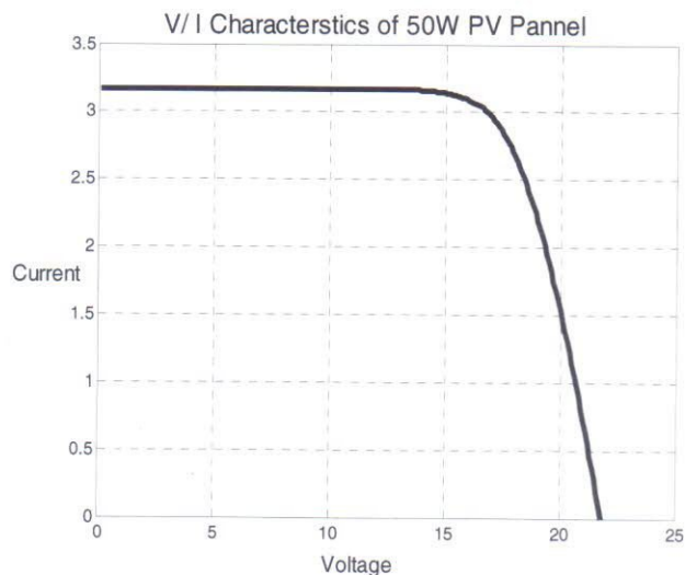
Fig. 2 Characteristics of BP 350 solar module at insolation 1000\text{W/m}^2 at 25^\circ\text{C}
