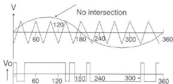
Fig. 3 Over modulation, = 1.3
