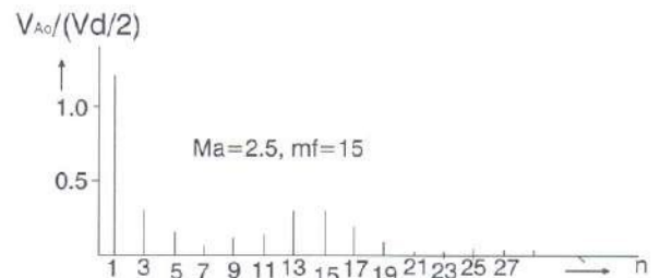
Fig4b Harmonics due to over modulation
