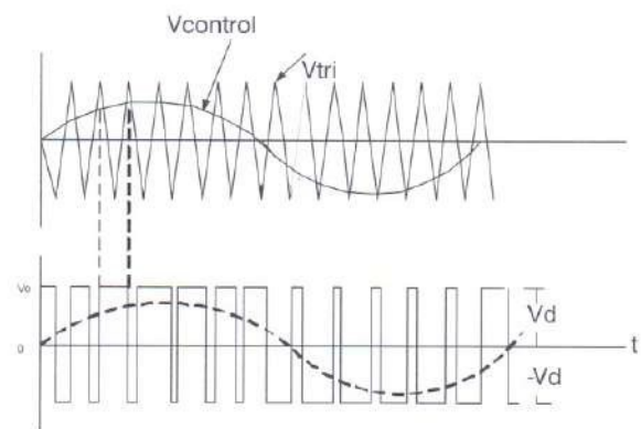
Fig 5 PWM with bipolar voltage switching
