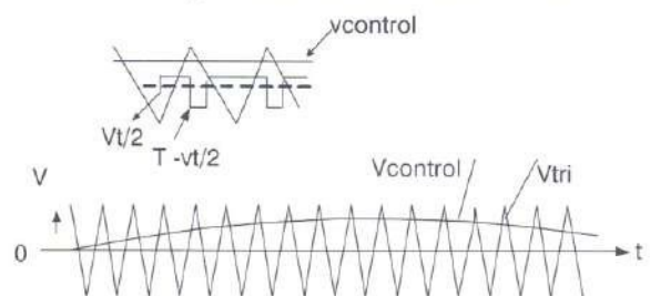
Fig4C Sinusoidal PWM
