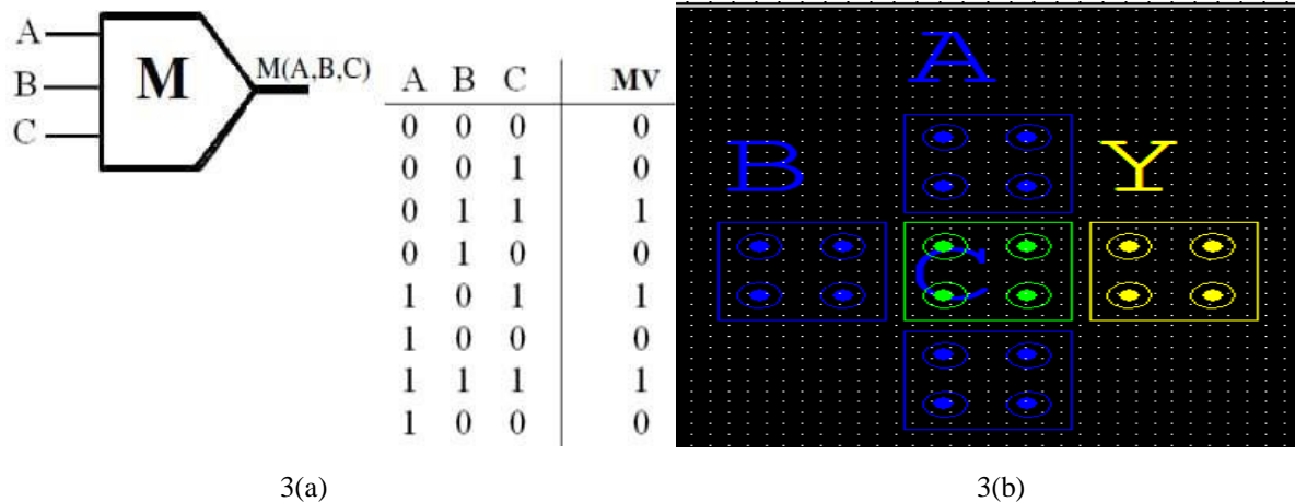
3(a) Block diagram of majority gate
