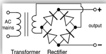
Figure 6 Step-Down Transformer
