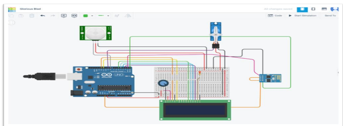
Figure 11. Implementation of Hardware on Tinker CAD Software
